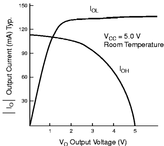
Figure 17. Output Drive Characteristics of EPF8282A Devices with 5.0-V V_{CC10}
